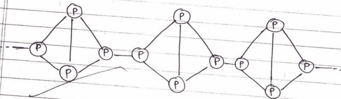
Structure of Red Phosphorus
