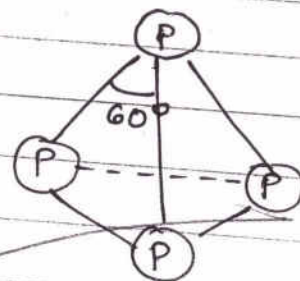
Structure of White Phosphorus
