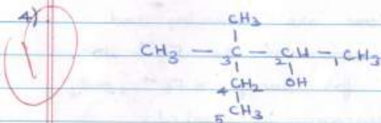
3,3-dimethyl pentan-2-ol
